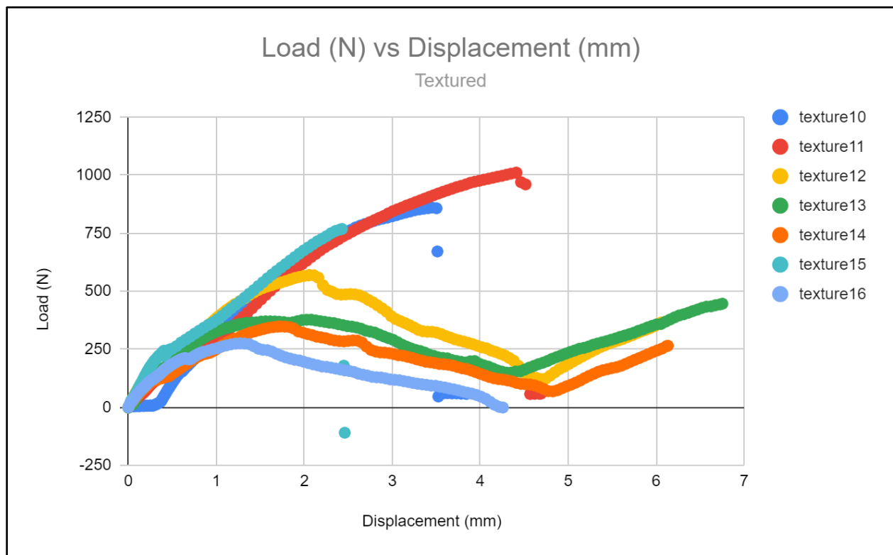
Figure 2: Tensile Testing Results for Textured 6-Hole Plates
