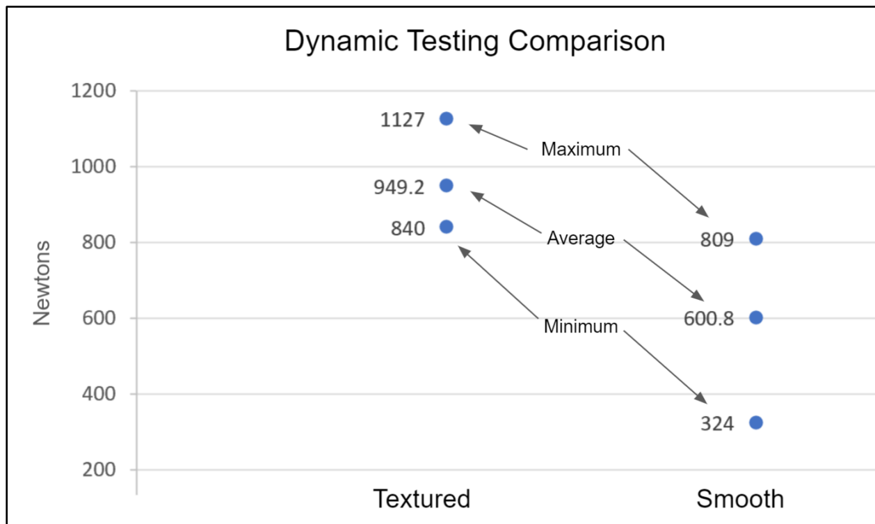
Figure 3: Dynamic Testing Results - Comparison between Textured and Smooth 1-Hole Plates
