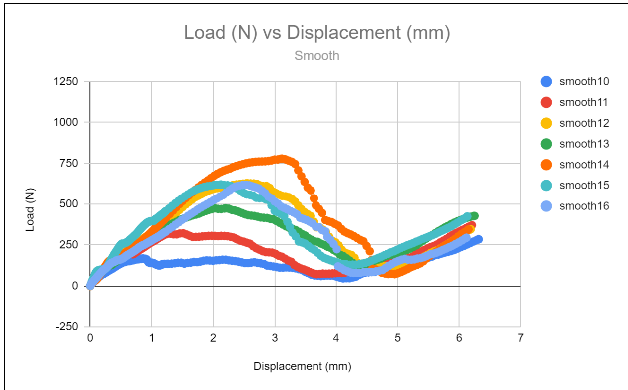
Figure 1: Tensile Testing Results for Smooth 6-Hole Plates
